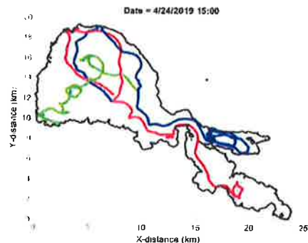
Fig. 7. Three-dimensional lake model results of possible pathways for particles. We used a different color to trace the path of each particle
