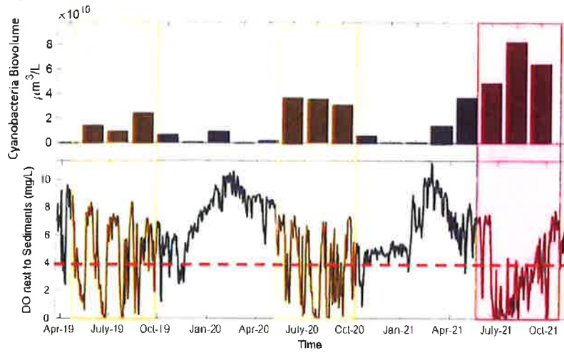
Fig. 1. (Top) Cyanobacteria biovolume from our in-lake sampling every 6-8 weeks in the Oaks Arm. (Bottom) Continuous-time series of benthic dissolved oxygen in the Oaks Arm. The red dashed line marks one of the possible DO thresholds to define hypoxia. The squares mark the summer periods when the cyanobacteria biovolume increases and the DO decreases
